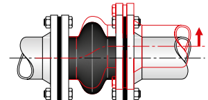
LATERAL DEFLECTION
