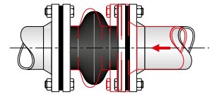
AXIAL COMPRESSION
